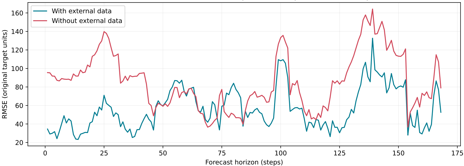
Final evaluation: six fold/seed squared errors pooled at each step
